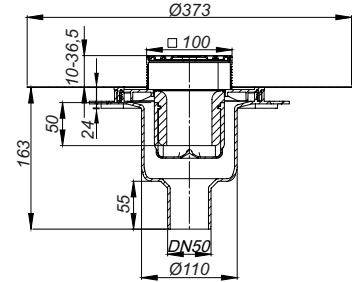
Sumidero DallDrain Select vertical OM, 100 x 100 mm
