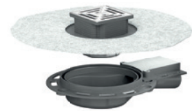
Sumidero DallDrain Select Plan ABS OM, 100 x 100 mm
