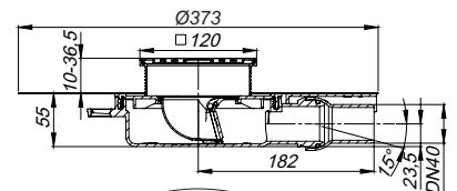
Sumidero DallDrain Select Plan ABS OM, 120 x 120 mm
