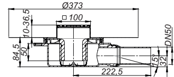
Sumidero DallDrain Select ABS OM, 100 x 100 mm
