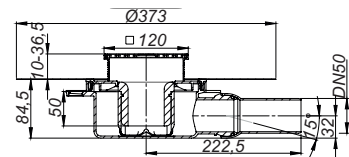
Sumidero DallDrain Select ABS OM, 120 x 120 mm
