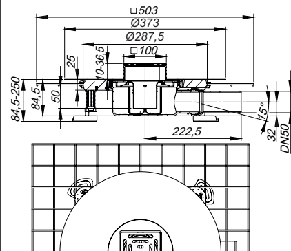
Sumidero CeraDrain Select, 100 x 100 mm
