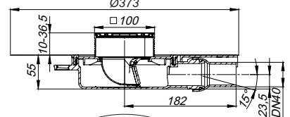
Sumidero DallDrain Select Plan ABS OM, 100 x 100 mm
