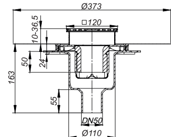
Sumidero DallDrain Select vertical OM, 120 x 120 mm
